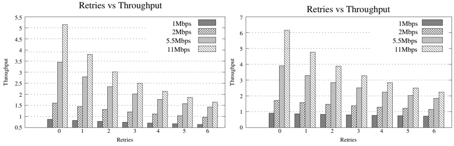
Fig. 3. Retries vs Throughput (RCS, Pksize=512 and 1024)
