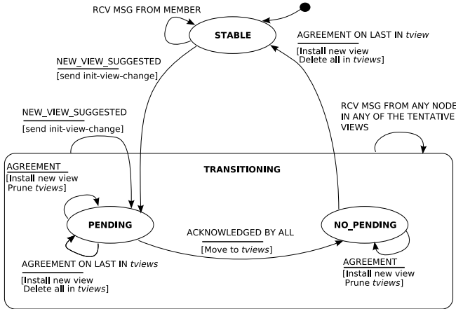
Fig. 2. State transition diagram for membership protocol
