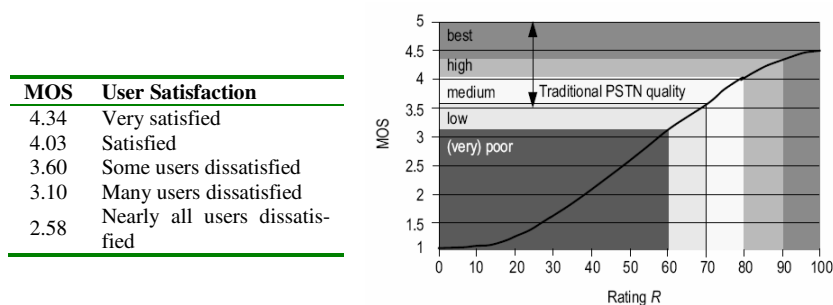
Fig. 3. MOS, Rating factor and user satisfaction taxonomy
