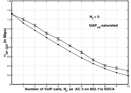
Fig. 11. Analysis and simulation results showing total download throughput obtained by QSTAs for different values of N_v and N_t = 5
