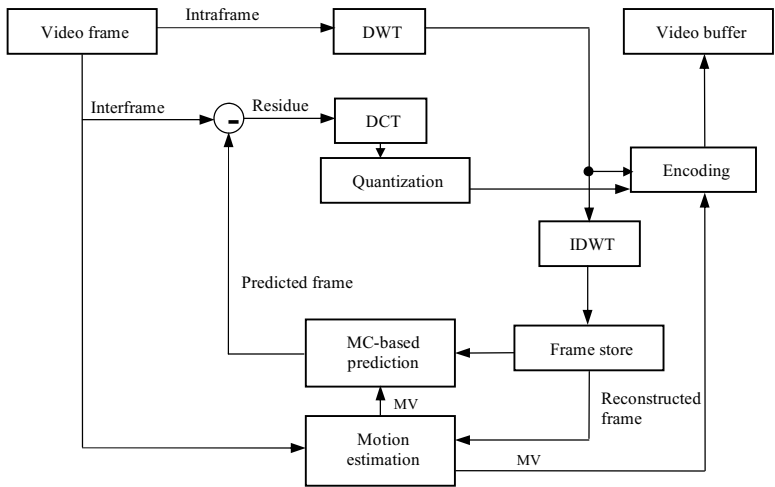
Fig. 3. Hybrid transform video encoder
