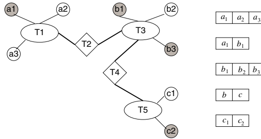
Fig. 2. E-R diagram corresponding to the example in section 4.2 and its tabular form
