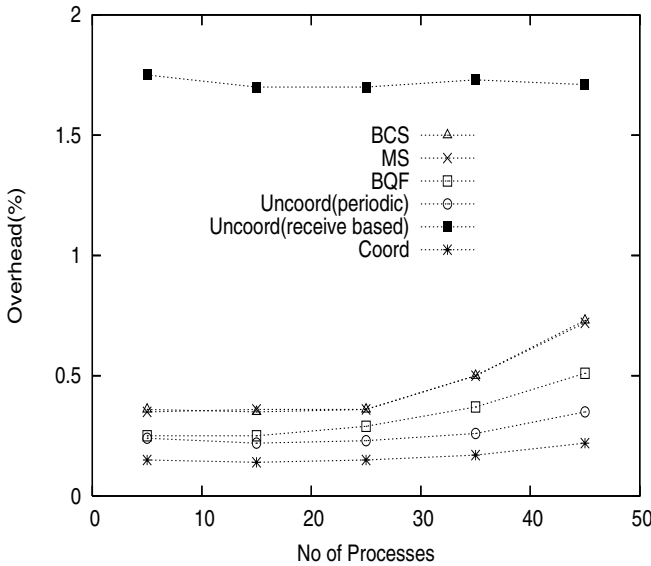
Fig. 1. Comparison of Checkpointing Overhead between different Algorithms
