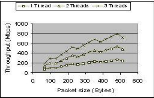
Fig. 5. Throughput variation
