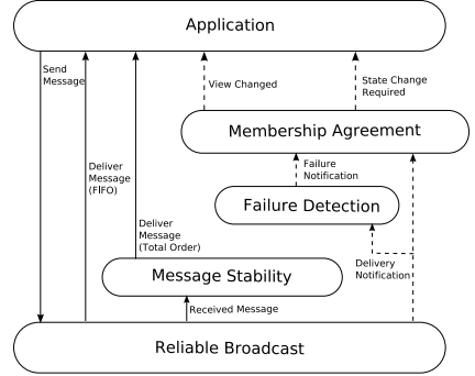
Fig. 1. TransMAN architecture
