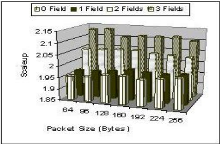
Fig. 6. Throughput scale-up for two threads
