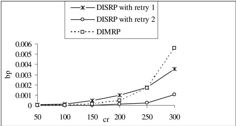
Fig. 1. Variation of bp with cr for DIMRP and DISRP (with retry) for w=70
