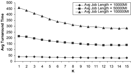
Fig. 13. Average turnaround time in the k -BudgetOptimized policy for different k
