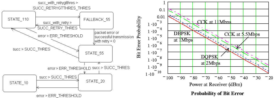
Fig. 4. (a) Rate Switching state diagram (b) Receiver Power vs BER
