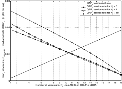
Fig. 5. Analysis results showing the service rate \Theta_{AP-VolP} applied to QAP_v , plotted vs. the number of voice calls, N_v for different number of TCP sessions N_t . Also shown is the line N_v \lambda . (From [6] © IEEE)
