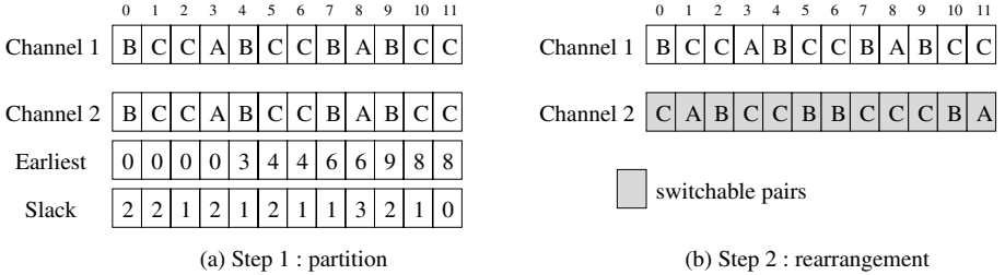
Fig. 3. Scheduling procedure
